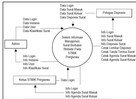
Gambar 2. Context Diagram
